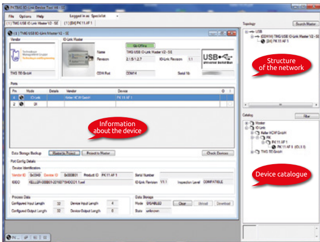
Fig. 5 Connection of an IO sensor to the master.
