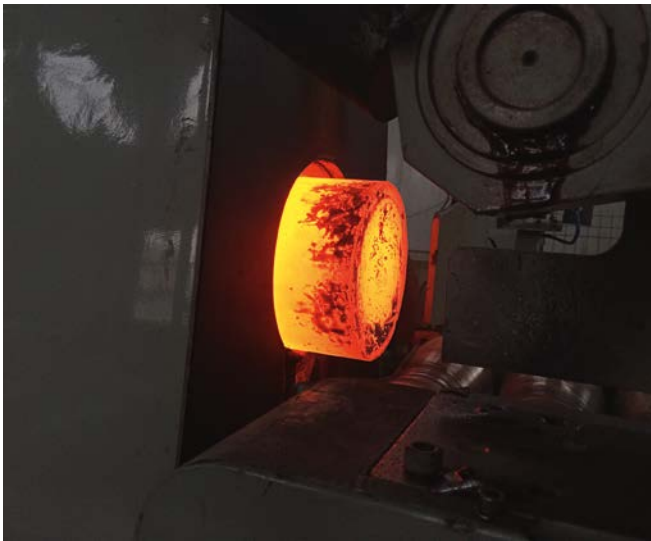
Fig. 6 Radiation ability of the forging block is extremely changed by scaling.
