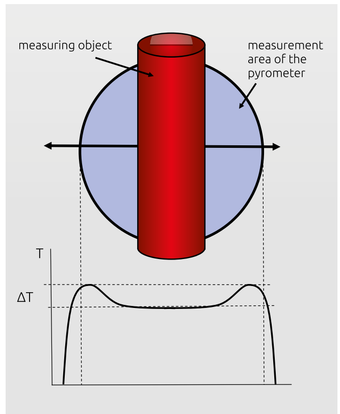
Fig. 5 Incorrect temperature increase when the hot object is located in the peripheral area of the target spot (measurement with a two-colour radiation pyrometer with a low quality lens).
