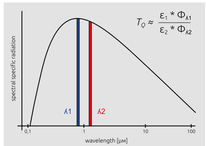
Fig. 1 Two-colour pyrometers measure the radiation at two wavelength ranges and determine the temperature from the ratio of the density of the radiation.
