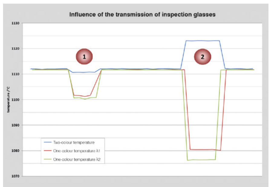
Fig. 4 Comparative measurement of the temperature variation for a high-quality protective glass (1) and a low-grade laminated glass (2).
