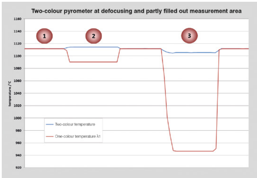
Fig. 6 Influence of the measuring distance on the two-colour and spectral temperatures.
