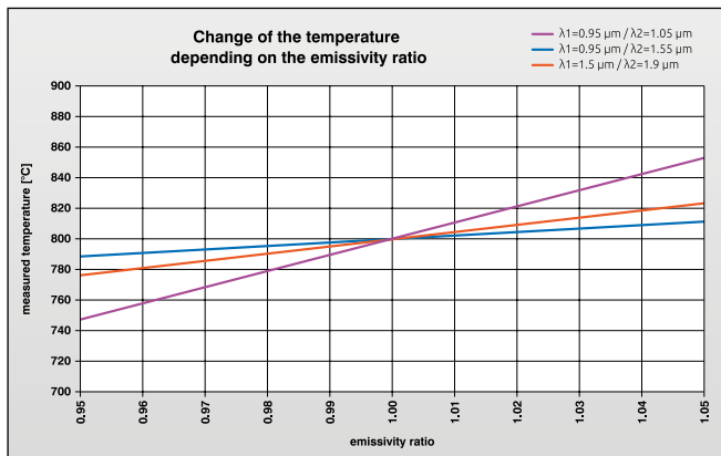
Fig. 2 Influence on the displayed temperature with a changing emissivity ratio of the target object at different wavelengths, based on an object temperature of 800 °C.
